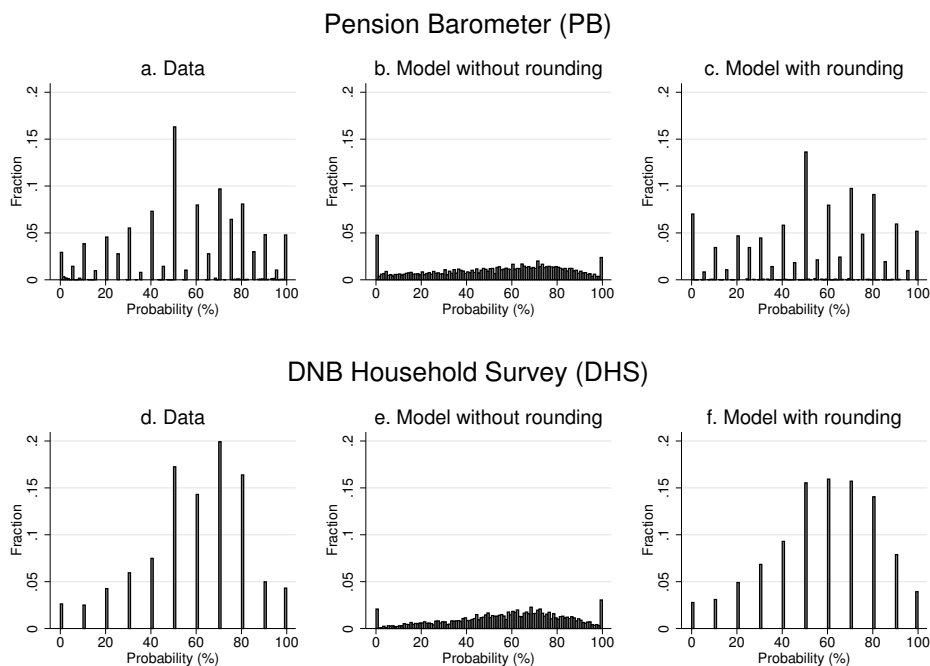
Figure 4: Histograms of data and simulated probabilities
