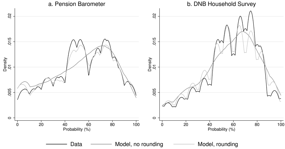
Figure 5: Kernel densities of data and simulated probabilities
