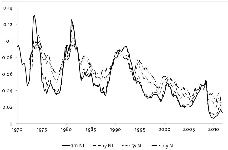
Figure 1: Nominal yields NL duration 3 month, 1, 5 and 10 years
