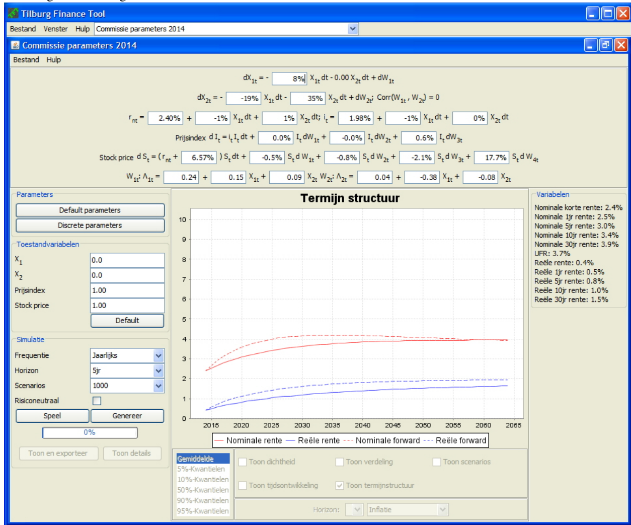
Figure 4: Settings TFT consistent with Dutch Committee Parameters 2014
