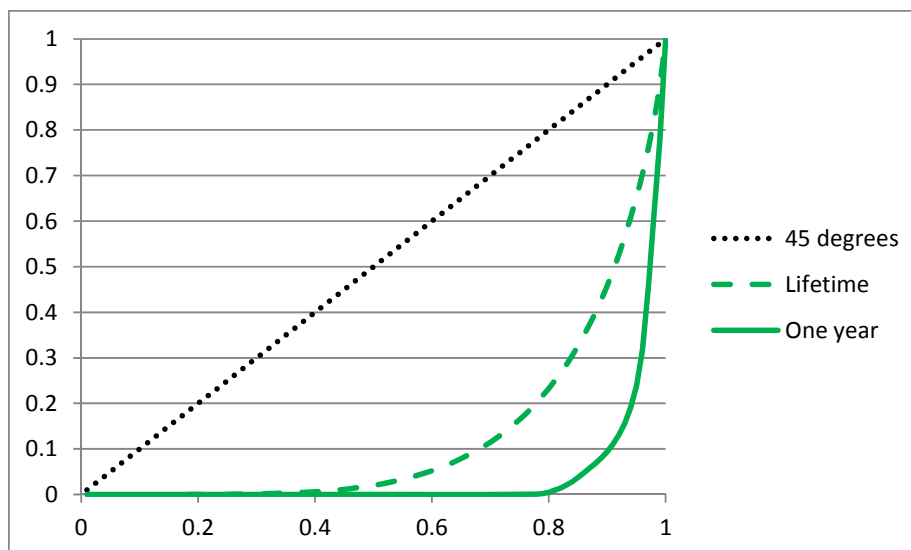
Figure 6: Lorenz curve for LTC costs measured per year and measured over the remaining lifetime at the age of 65
