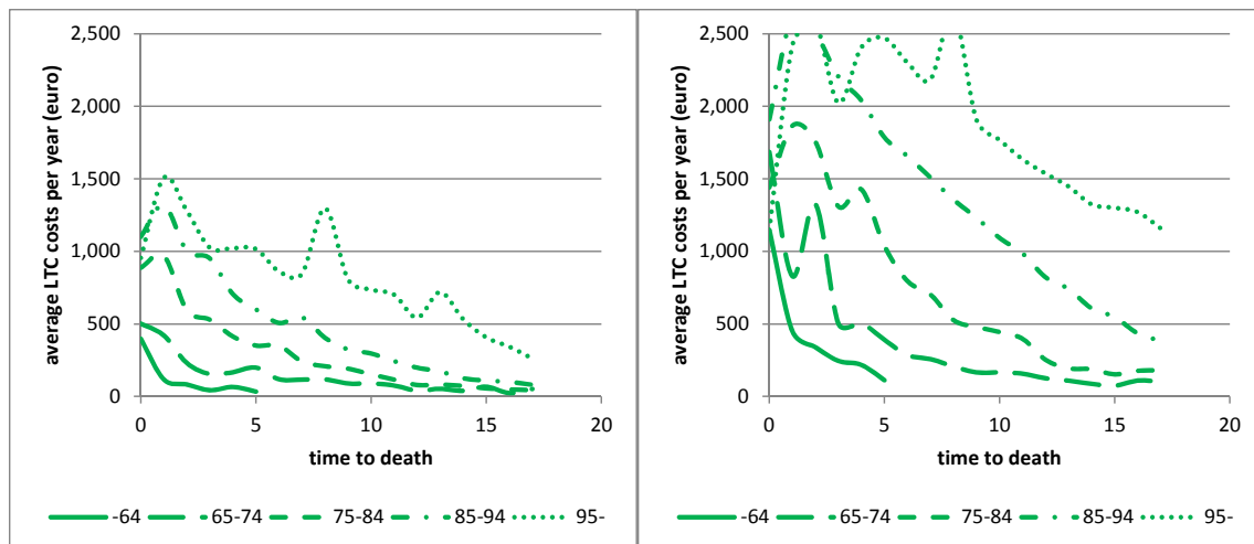
Figure 5 Average extramural LTC costs per annum before death (time to death) per group with different ages at death, males (left), females (right)
