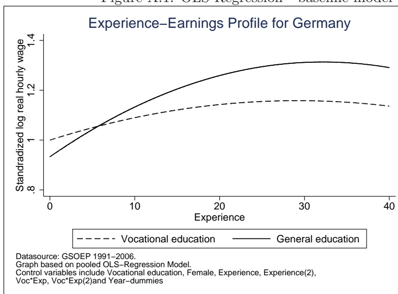
Figure A.1: OLS-Regression - baseline model
