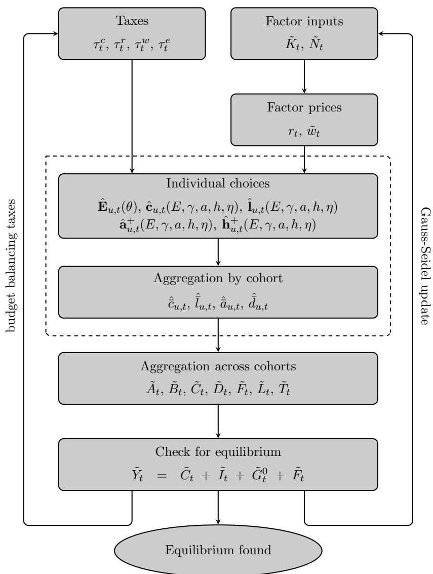
Figure C.1: Program structure
